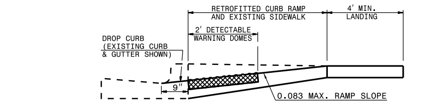
SECTION B-B
